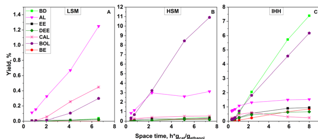
Fig. 6 Effect of space time on the conversion of ethanol at 350 °C over the (A) LSM, (B) HSM and (C) IHH catalysts. The WHSV of ethanol was varied between 0.2 and 3.0 g ethanol g cat -1 h -1 . Otherwise, standard reaction conditions were used.
