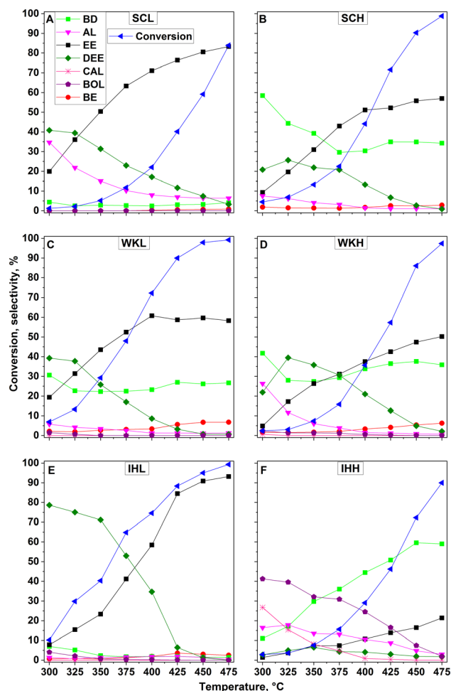
Q15 Fig. 3 Catalytic conversion of ethanol at different temperatures over the MgO-SiO 2 catalyst preparations, having a Mg to Si ratio of 2 to 1 under standard reaction conditions, such as atmospheric pressure, 15 kPa ethanol/He, 0.5 g ethanol g cat -1 h -1 , and a total gas flow rate of 30 ml min -1 .
