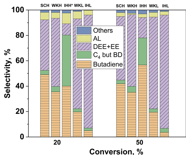
Fig. 7 Product distribution at 20 and 50% conversion levels over different MgO-SiO 2 catalysts. Identical conversions with the catalysts of different activities were achieved by adjusting the ethanol WHSV between 0.2 and 3.0 g ethanol g cat -1 h -1 at about a 15 kPa partial pressure at 350 °C for 20% conversion and 400 °C for 50% conversion. *Over the IHH sample, the attained maximum conversion was only ~18%. Others: methane, propylene, higher olefins.
