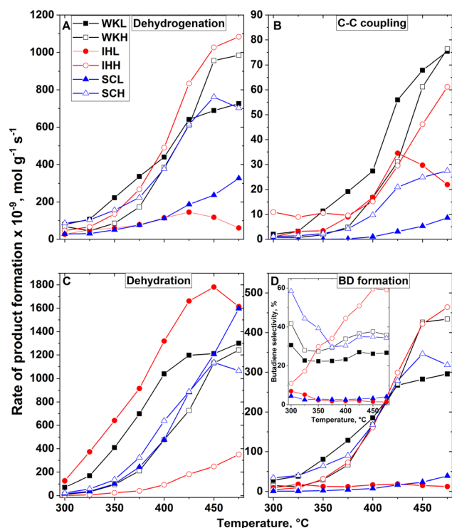
Fig. 4 Formation rates of ETB reaction products obtained by (A) dehydrogenation to AL, (B) C-C coupling to ΣC 4 products (BOL, BE, CAL) but not to BD, (C) ethanol dehydration (EE plus DEE), and (D) C-C coupling to BD as a function of reaction temperature under standard reaction conditions. The insert in section (D) shows the butadiene selectivities. The rate of dehydrogenation was calculated as the rate of Al formation plus twice the rate of ΣC 4 formation.
